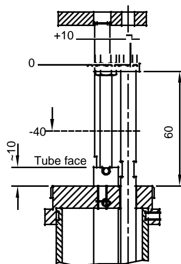
Upward borehole
