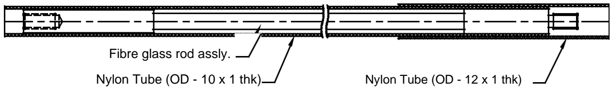
Figure 2.3 – Fibreglass connecting rod assembly
