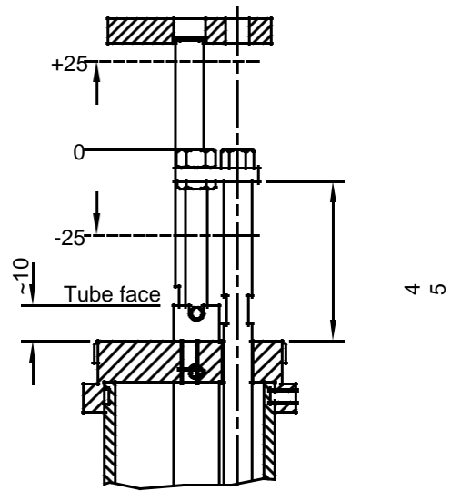
Mid position borehole
